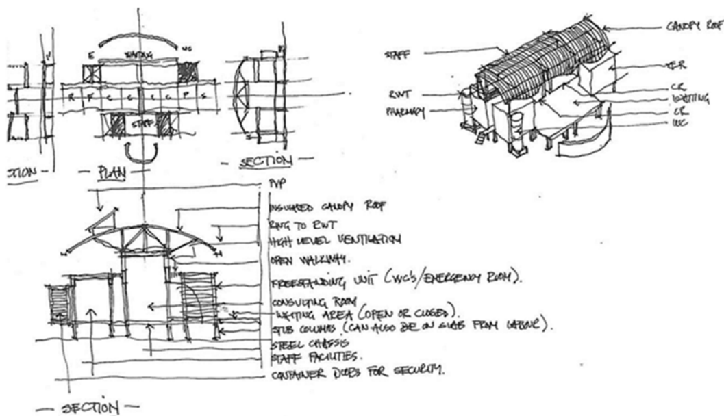
Figure 3: Design sketch
