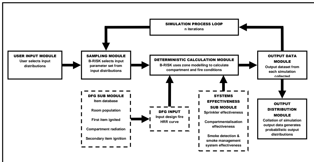
Figure 1: Schematic structure of B-RISK modules.
