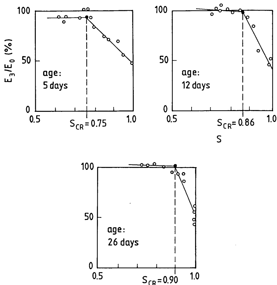
Fig. 2: The critical degree of saturation of a certain concrete as function of the concrete age. The parameter E_3/E_0 is the ratio dynamic E-modulus after 3 freeze-thaw cycles and before freeze-thaw
